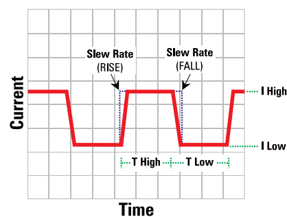
Fig.4 - Dynamic Mode for DC models
