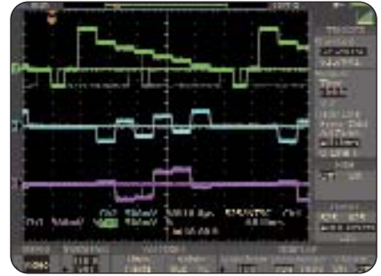
► Trace and identify ITU-R BT.601 video signals with the TDS3SDI 601 Serial Digital Video Module.
