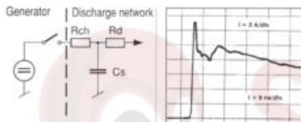
Simple equivalent circuit
