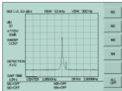
In-Band Spur Measurement
