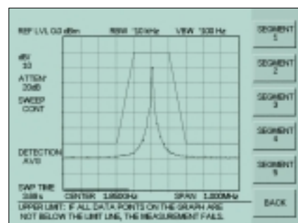
Segmented Limit Line
