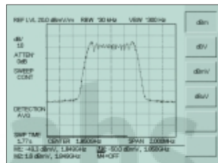
Field Strength Measurement
