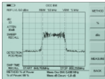
Occupied Bandwidth Measurement
