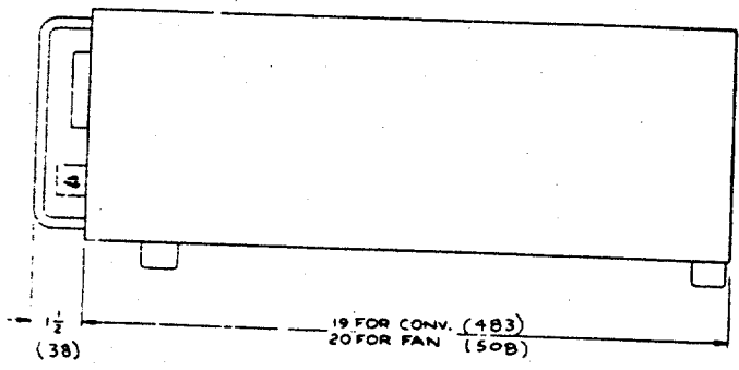
Figure 6-18 DCR-B 2700W Outline Drawing (Except 7-300B)
