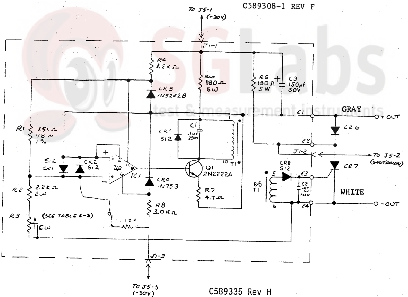
Figure 6-16 OVP Schematic and Component Location (All Models Except 7-300B)
