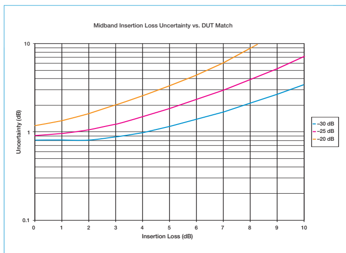
S820D Insertion Loss Uncertainty vs. DUT Match, Frequency = 10 GHz
