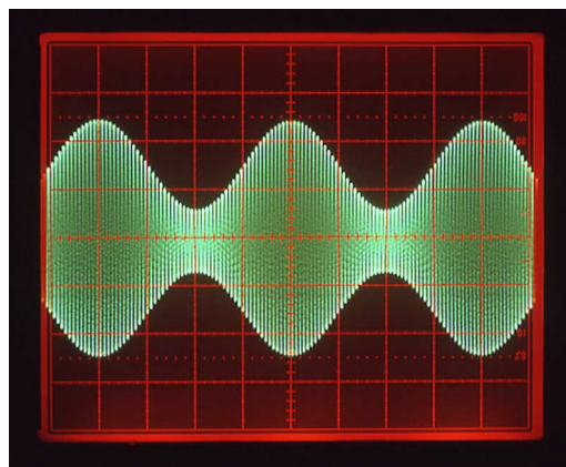
Amplitude modulation
