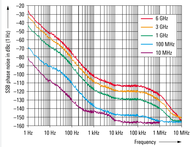
Measured SSB phase noise with internal OCXO
