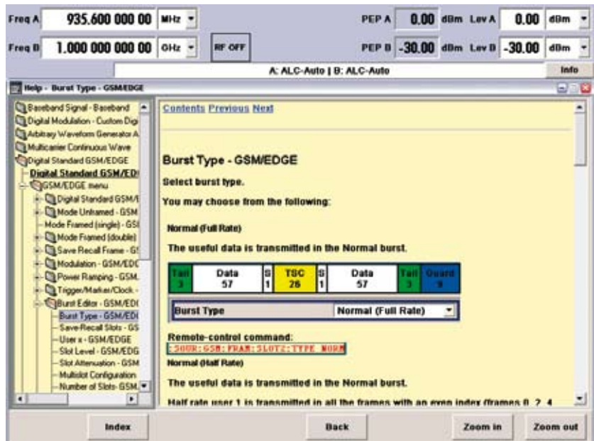
Help system
