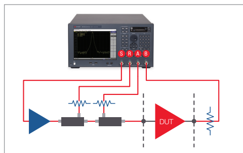
High-power measurement using external test set mode
