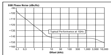
Typical phase noise performance at 1 GHz
