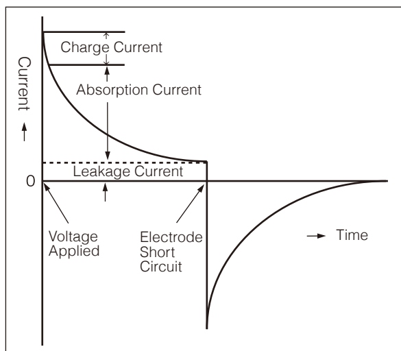
Absorption Current Characteristic Curve
