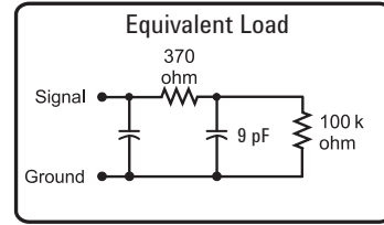
Figure 3.25. Suggested on-board isolation network and equivalent load when using discrete components to terminate the E5351A
