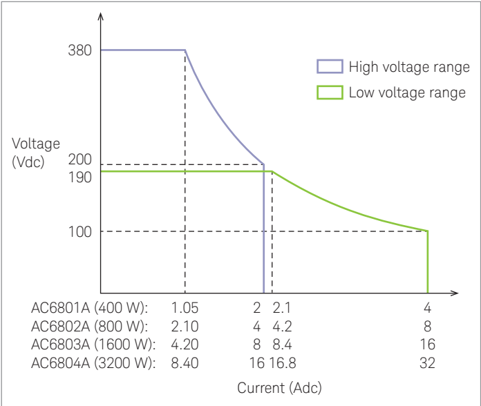
AC6800 steady-state DC output characteristic
