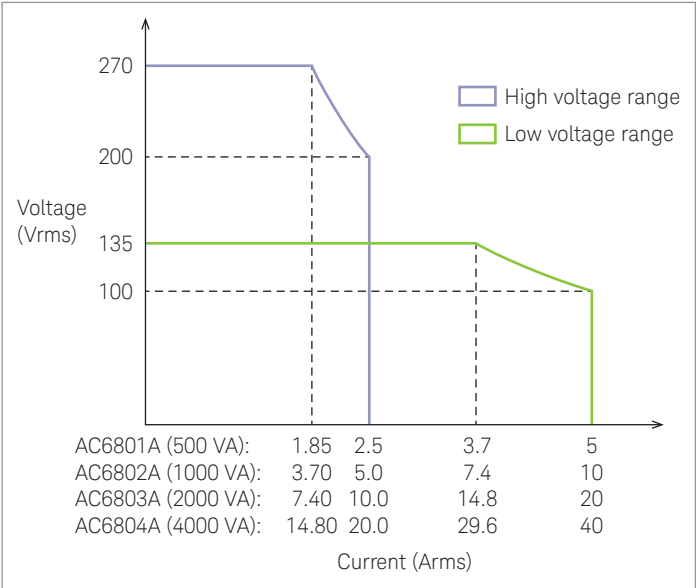
AC6800 steady-state AC output characteristic
