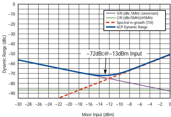
< Dynamic Range of W-CDMA Measurement (5MHz offset) >
