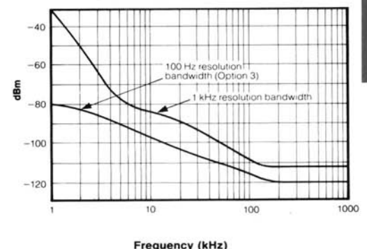
Typical low end frequency performance for the 492 with Option 03.
