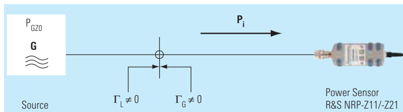
FIG 3: \Gamma correction function: By taking into account the complex reflection coefficient \Gamma_G of the source, the measurement result ( P_i ) is corrected in such a way that the nominal power of the source P_{GZ0} is displayed.
