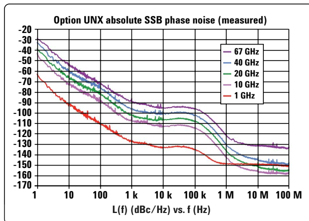
Option UNX phase noise
