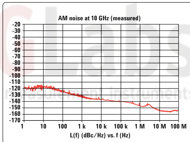
AM noise at 10 GHz
