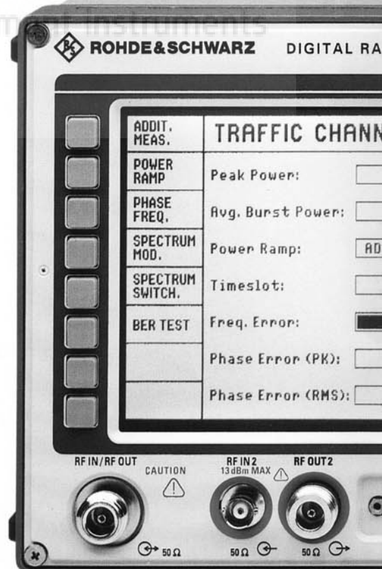
Digital Radiocommunication Tester CMD 57 with options
