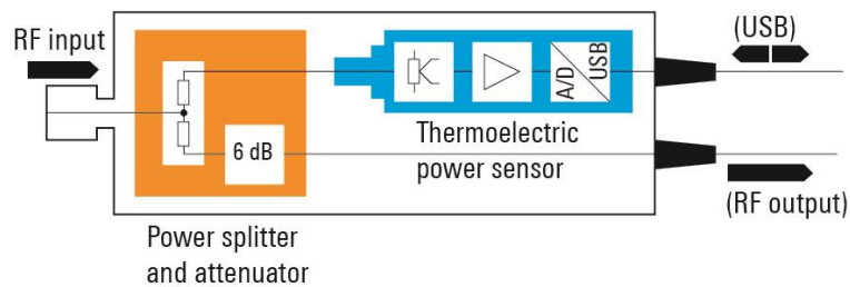
Block diagram of the R&amp;S®NRP-Z27/-Z37 power sensor modules
