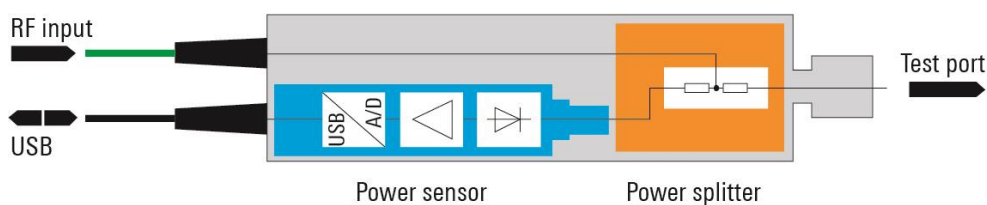
Block diagram of the R&S®NRP-Z28/-Z98 level control sensors
