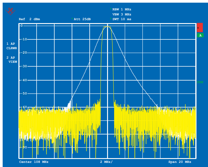
Comparison of 1 MHz channel filter and normal 1 MHz resolution filter.
