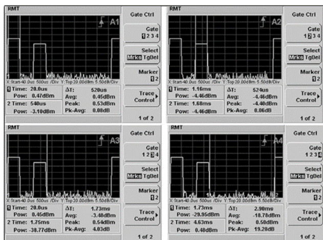
Figure 7. Measurement flexibility with 4 independent time gates
