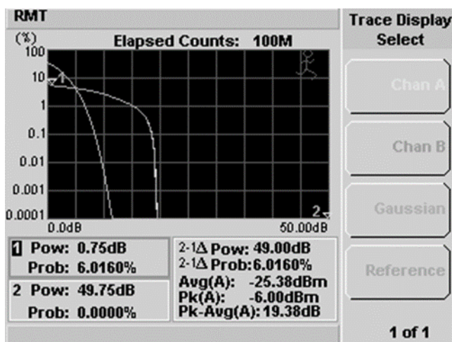
Figure 9. CCDF statistical measurements
