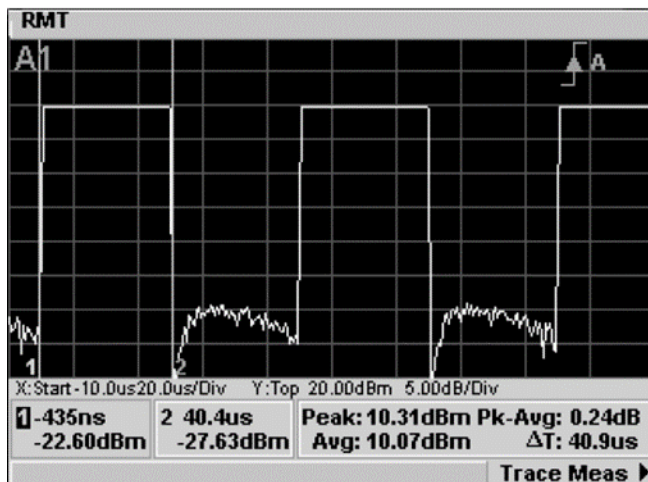
Figure 6. Comprehensive-time measurements: comprising rise time, fall time, pulse width, pulse period, duty cycle, time to positive and negative occurrences and pulse repetitive frequency.
