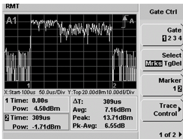
Figure 8. WiMAX burst signal capture
