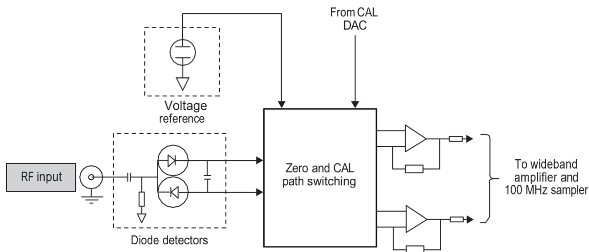
Figure 1. Internal zero and cal block diagram
