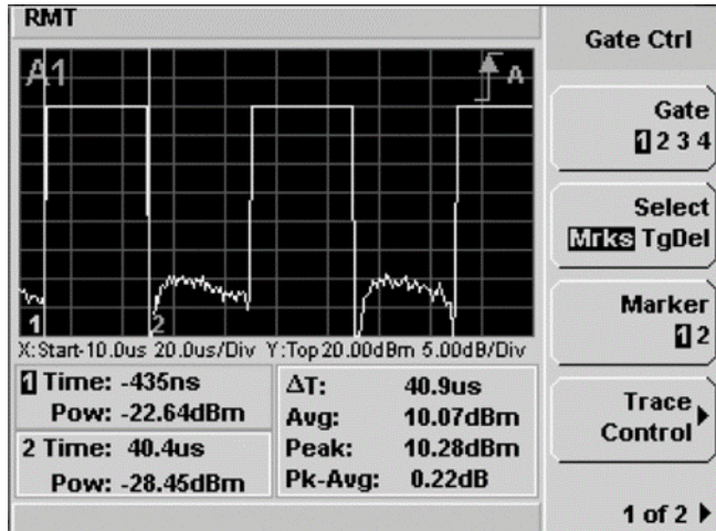
Figure 5. Markers 1 and 2 time and power, with \Delta time and power measurements between markers.
