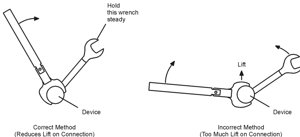
Figure 3-3 Wrench Positions
